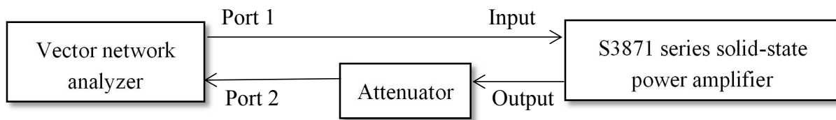
Figure 5-1 Gain and standing wave testing diagram
