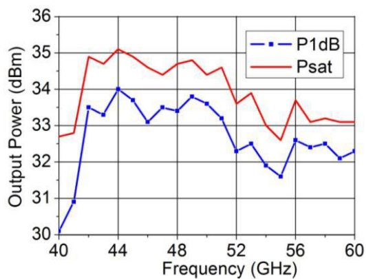
S3871LA Output power VS Frequency
